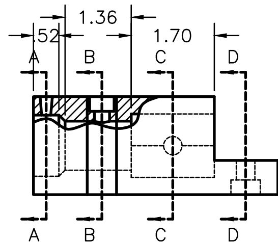
CASING SCALE 1:2
